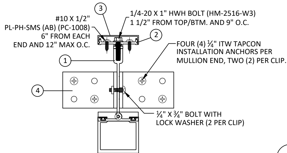
D 2 HORIZONTAL SECTION CONCRETE/MASONRY MULLION CLIP
